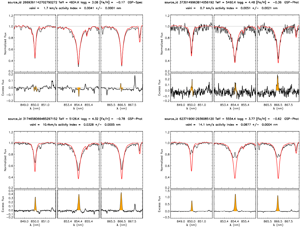
Fig. 5. Ca II IRT sample spectra in the different regimes. In each panel, the spectra (black line) are compared with the template (red line). The enhancement factor, i.e. the integrand of Eq. (1), is reported below the spectrum, and the integral producing \alpha is outlined in orange. Upper left panel: LA subgiant with \log R'_{\text{IRT}} = -6.04 . Upper right panel: LA dwarf with \log R'_{\text{IRT}} = -5.98 . Lower left panel: HA dwarf with \log R'_{\text{IRT}} = -5.19 . Lower right panel: accreting star (one in the Upper Scorpius association reported in Table 2 and Fig. 8) in the VHA regime.
