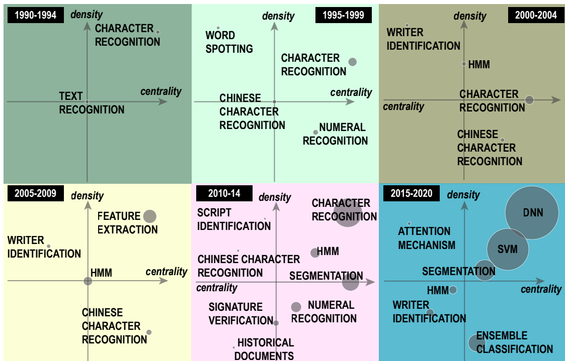
Figure 10: Strategic diagrams per period.
