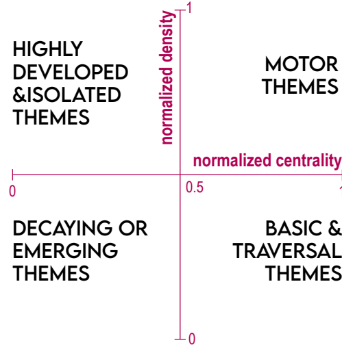
Figure 2: TN roles according to the strategic diagram quadrants.
